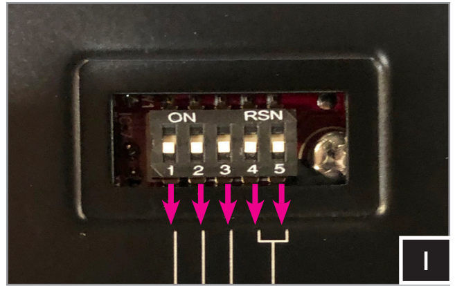
I. On bottom side of the 500.1 amp, remove switch cover, and set switch levels to match.
