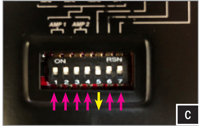
C. On bottom side of the 300.4 amp, remove switch cover, and set switch levels to match.
