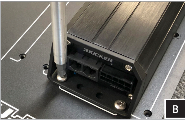
B. With the amplifier disconnected, unscrew the (4) screws that secure the amp to the amp tray.
