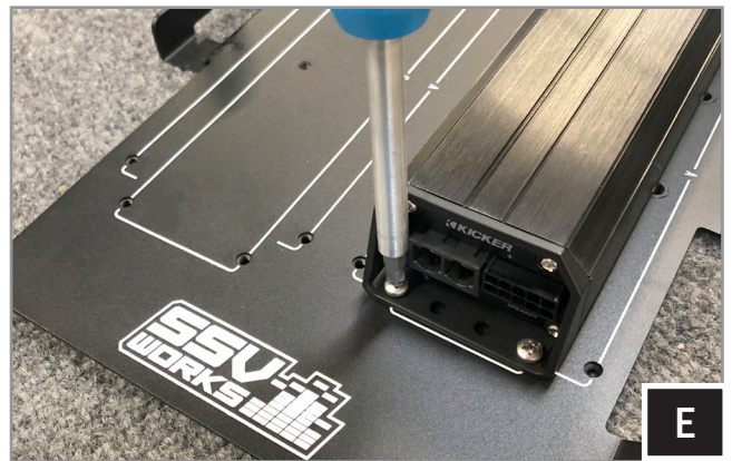
E. Transfer the 300.4 amp to the Ride Command compatible amp tray. Fasten the amp to the tray with your existing M4 hardware. We recommend applying Threadlocker.
