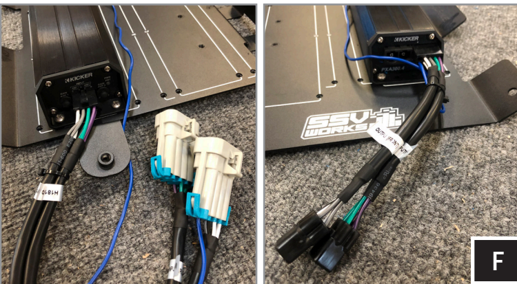
F. Connect harness B-H1810 to the 300.4. The 8-pin connector to the input side of the amp and 10-pin connector to the output side of the amp.
