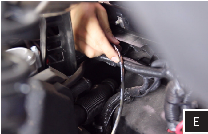
E. Route the rear speaker harness (B-H1150) along the factory wires in the engine compartment and pull up through the small space between the bed panel and cage tubing on both passenger and driver sides.
